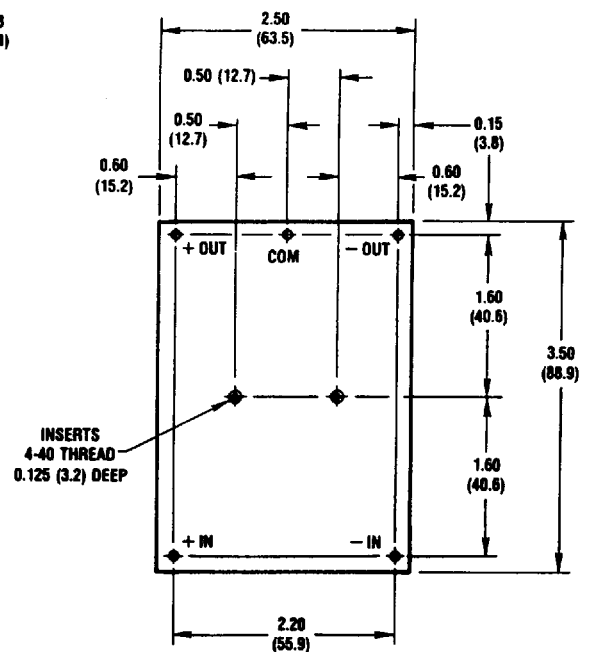
Bottom View
